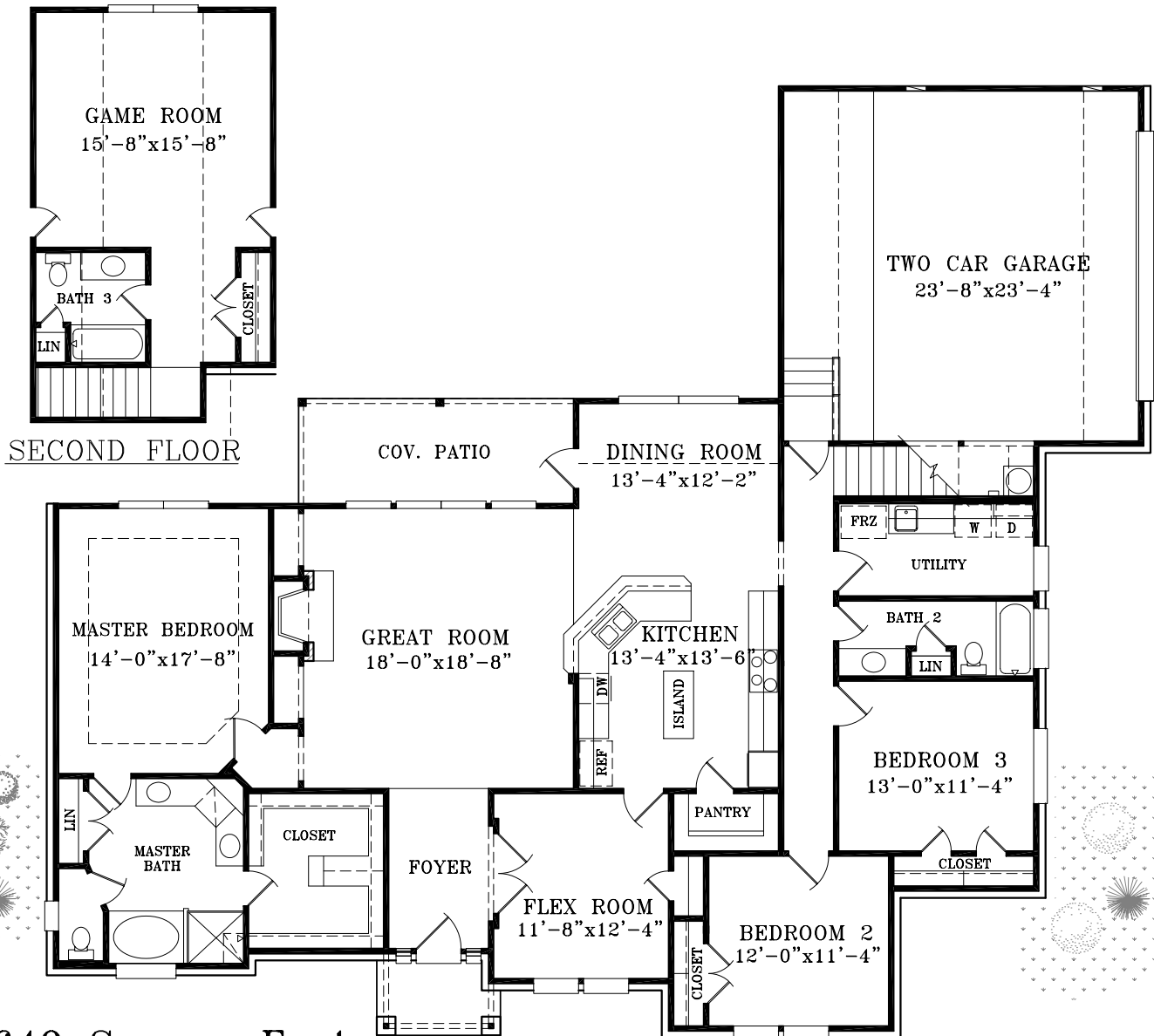
FLOOR PLAN
